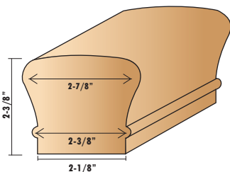
6210 Top Rail 2-3/8" x 2-7/8" 6210-101
