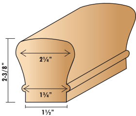
6010 Top Rail 2-3/8" x 2 1/4" 6010-101
