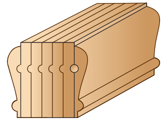
Colonial Bending Rail* 001-105 *use 001 bending mold
