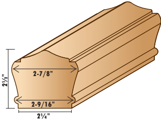
Lambton Top Rail
