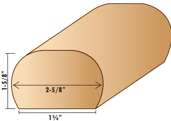
Oval Top Rail
